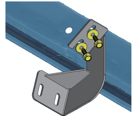
Center Passenger Side Bracket
