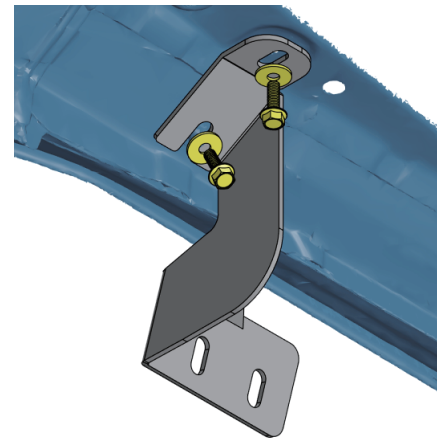
Front Passenger Side Bracket
