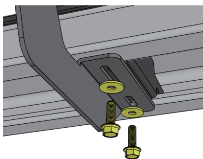
Stainless Steel Step Bar
